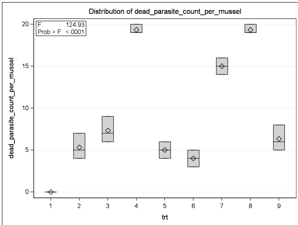
Fig 1: A box plot graph displaying the efficacy of different chemicals on leech of freshwater mussel, L. marginalis (X-axis: 1: Control; 2: T 1 , 3: T 2 , 4: T 3 , 5: T 4 , 6: T 5 , 7: T 6 , 8: T 7 , 9: T 8 )
