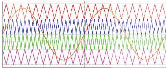
Figure 8.5. Waveform of POD-PWM with variable frequency
