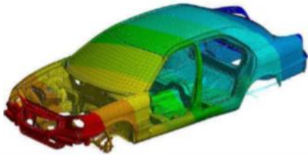
Meshing of Monocoque chassis
